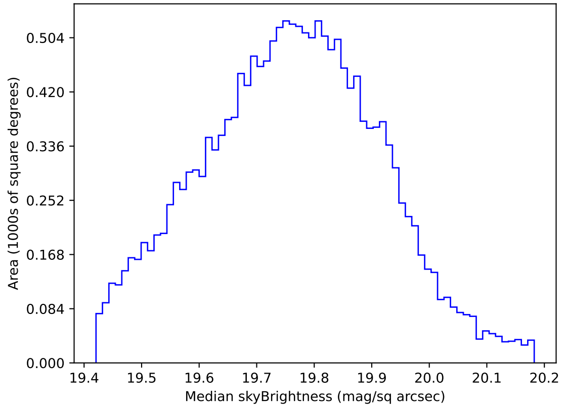
internal_u_expt60_nscale1.5v3.4_10yrs WFD all bands: Median skyBrightness
