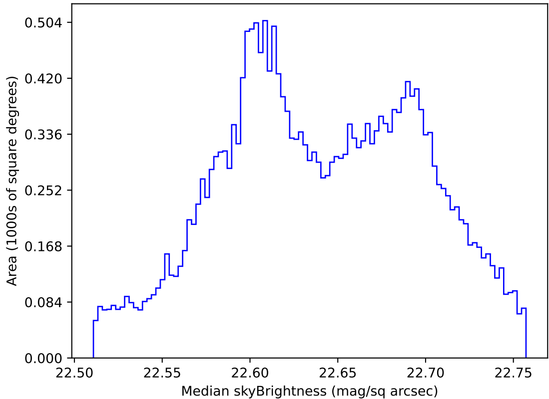
internal_u_expt60_nscale1.5v3.4_10yrs All sky u band: Median skyBrightness
