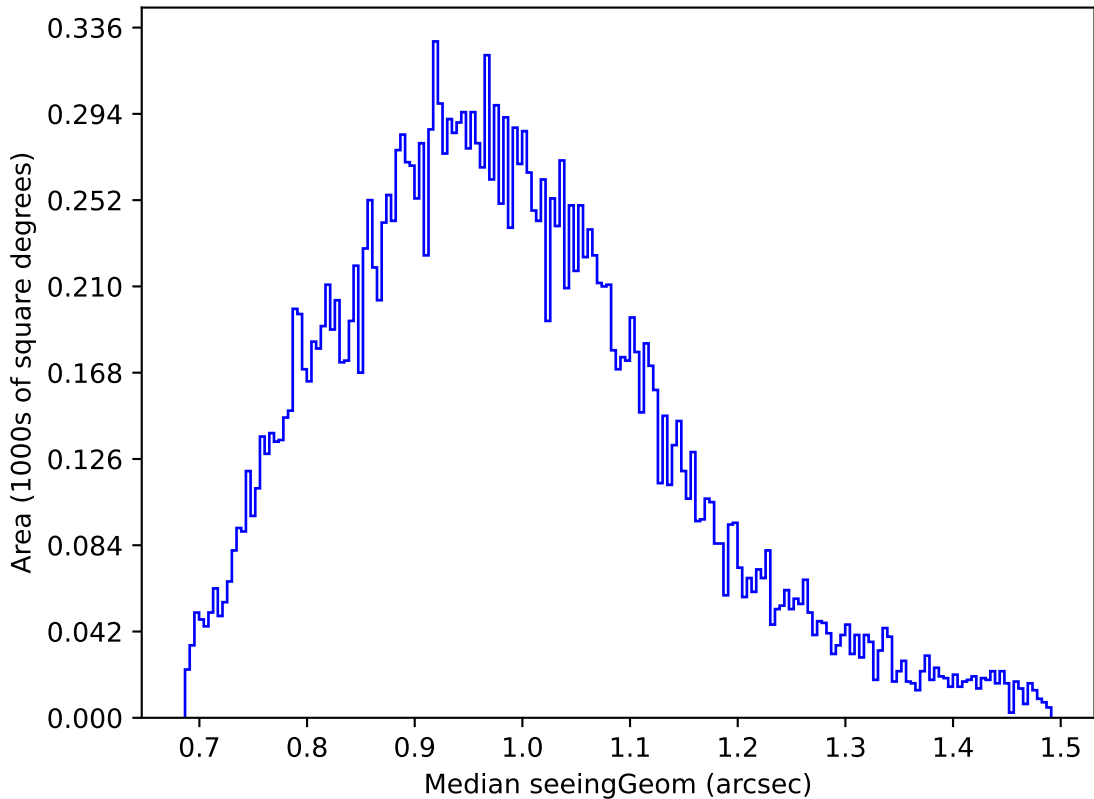
internal_u_expt60_nscale1.5v3.4_10yrs Yr 1 u band: Median seeingGeom
