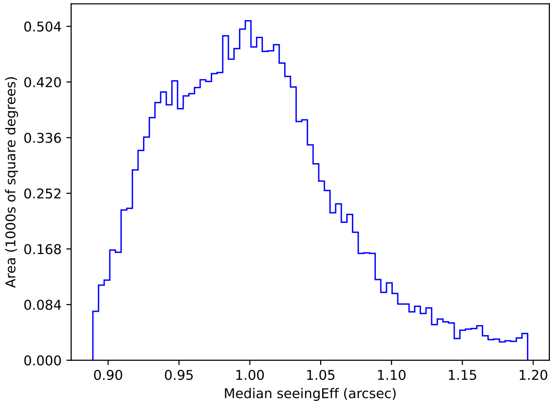
internal_u_expt60_nscale1.5v3.4_10yrs WFD y band: Median seeingEff
