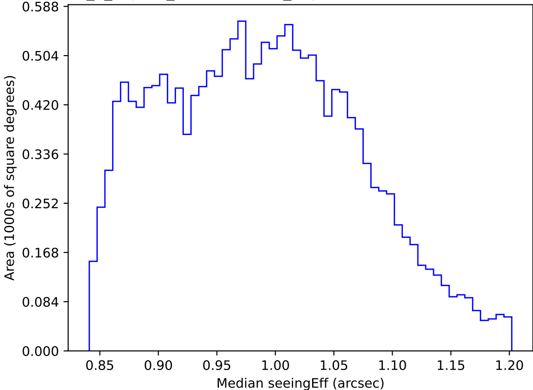
internal_u_expt60_nscale1.5v3.4_10yrs WFD i band: Median seeingEff
