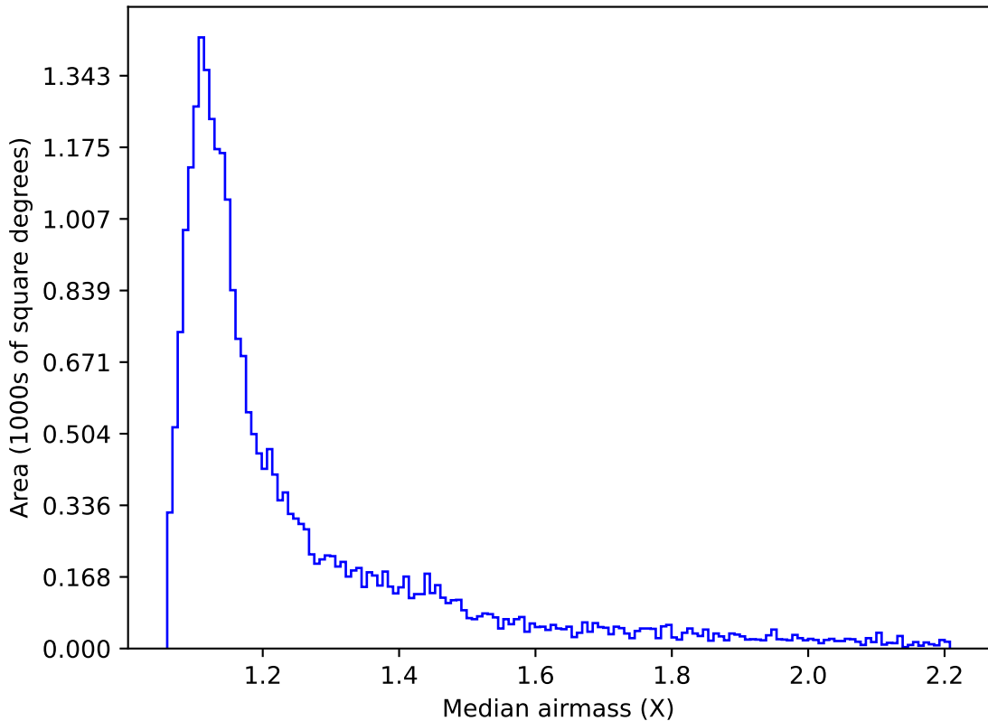
internal_u_expt60_nscale1.5v3.4_10yrs Yr 1 z band: Median airmass
