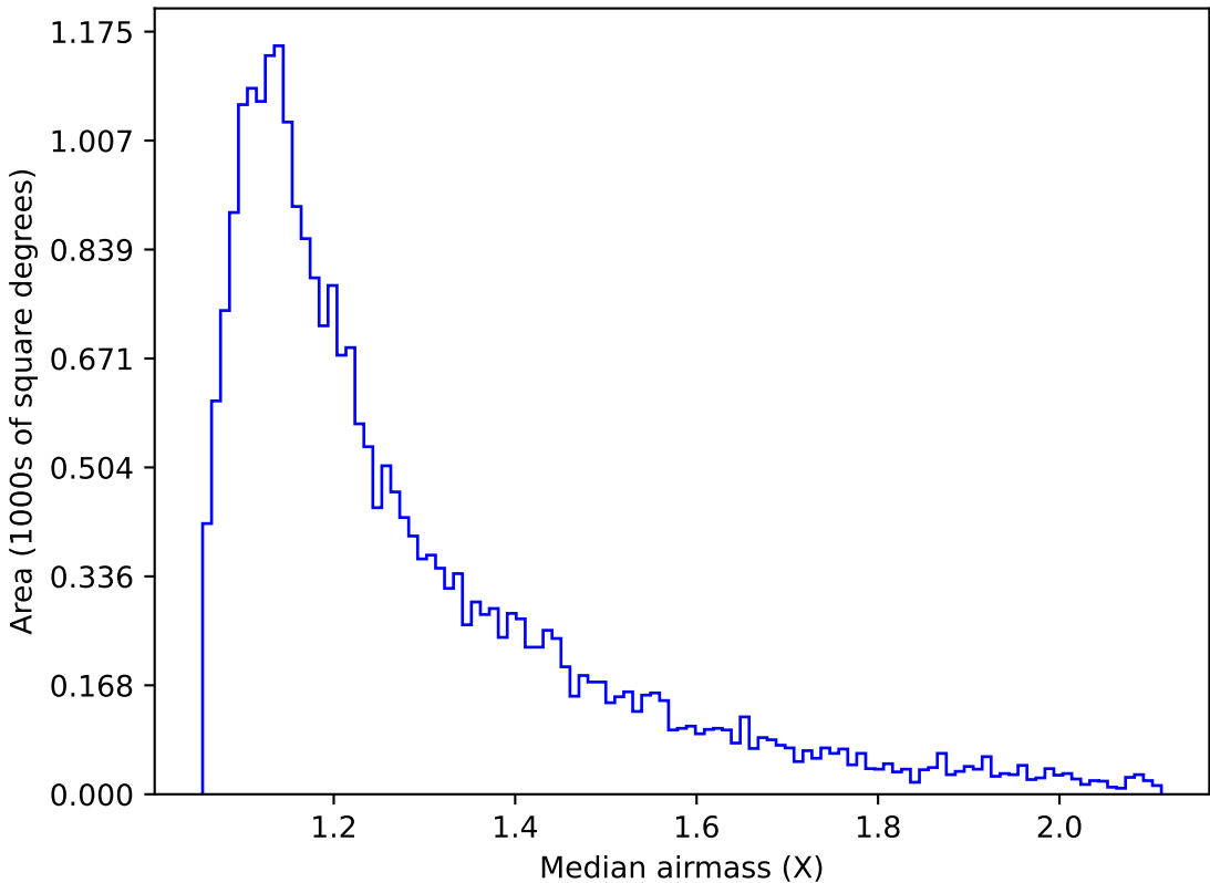
internal_u_expt60_nscale1.5v3.4_10yrs Yr 1 g band: Median airmass
