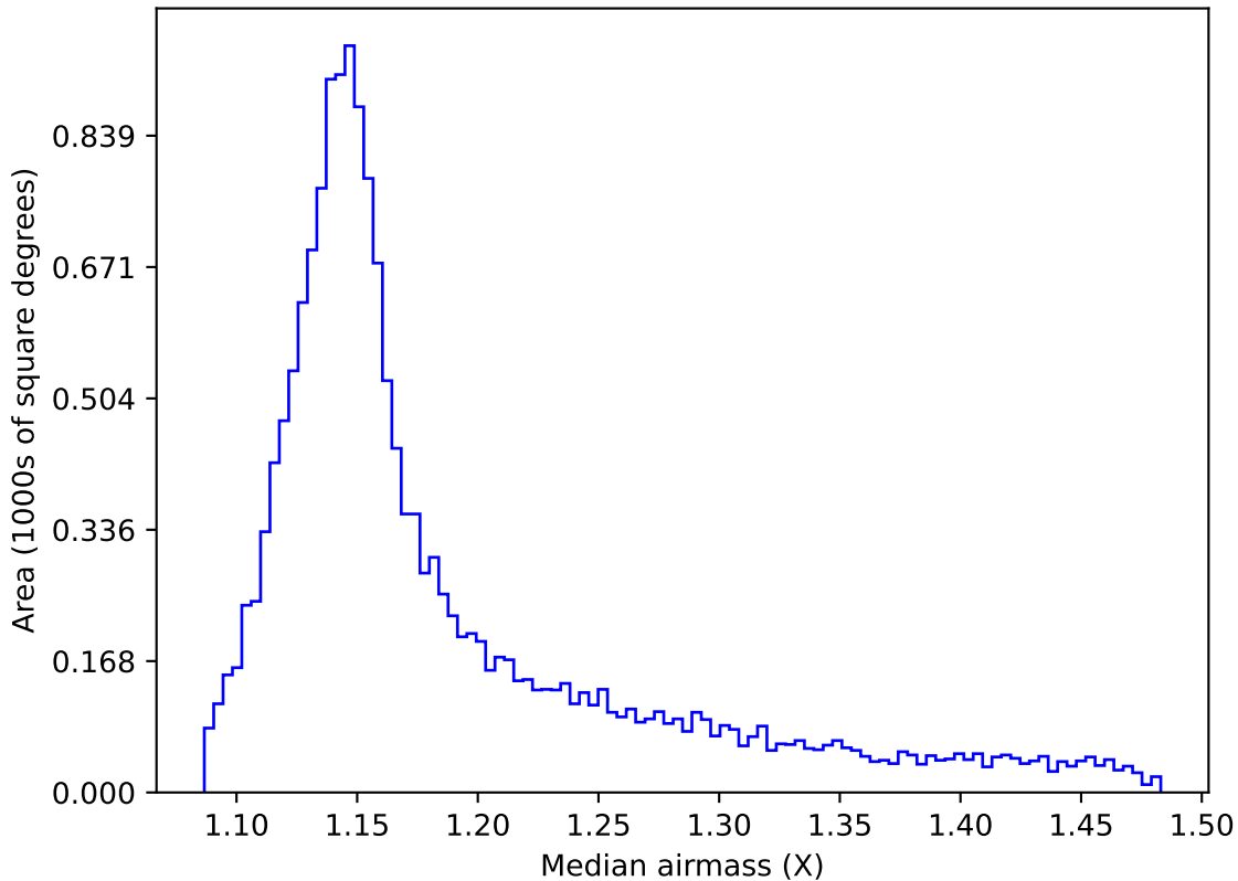
internal_u_expt60_nscale1.5v3.4_10yrs WFD y band: Median airmass
