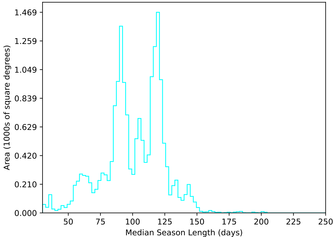
internal_u_expt60_nscale1.5v3.4_10yrs WFD u band: Median Season Length
