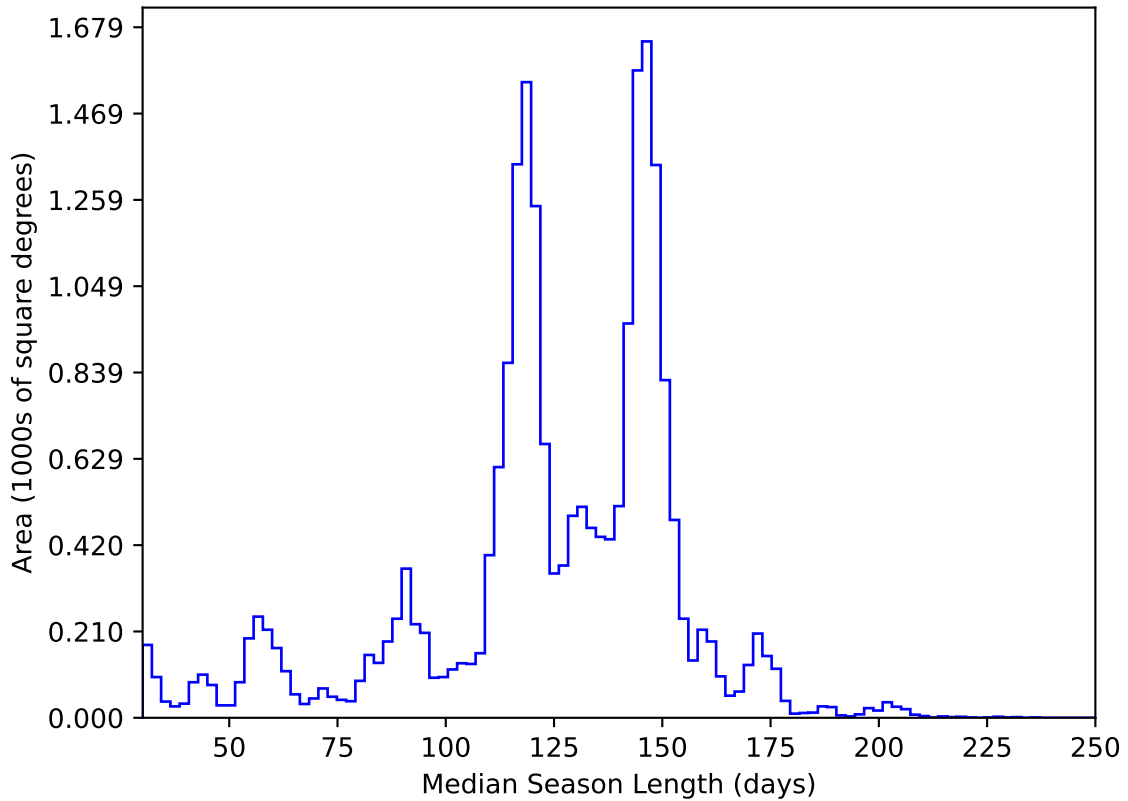
internal_u_expt60_nscale1.5v3.4_10yrs All sky y band: Median Season Length
