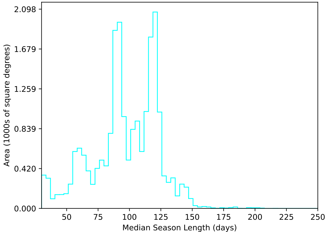
internal_u_expt60_nscale1.5v3.4_10yrs All sky u band: Median Season Length
