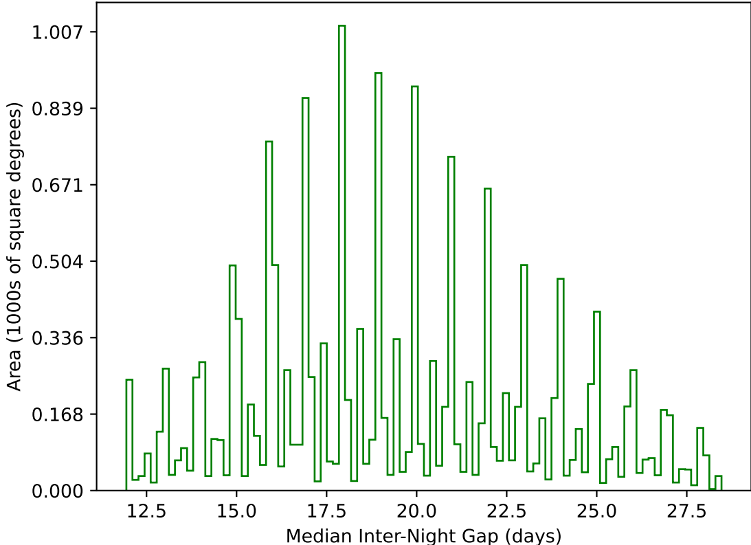
internal_u_expt60_nscale1.5v3.4_10yrs WFD g band: Median Inter-Night Gap
