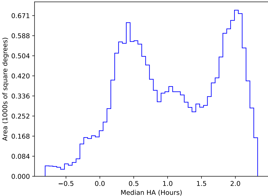
internal_u_expt60_nscale1.5v3.4_10yrs WFD z band: Median HA
