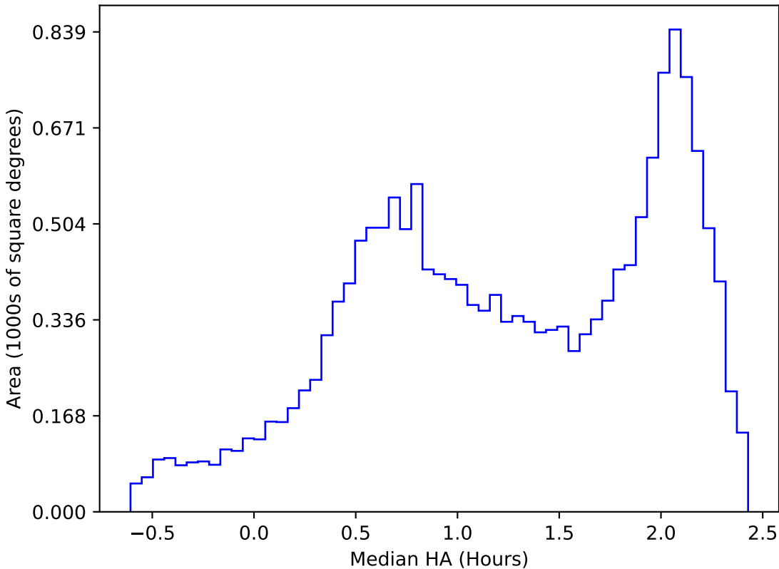
internal_u_expt60_nscale1.5v3.4_10yrs WFD y band: Median HA
