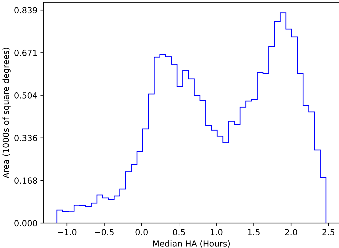
internal_u_expt60_nscale1.5v3.4_10yrs WFD u band: Median HA
