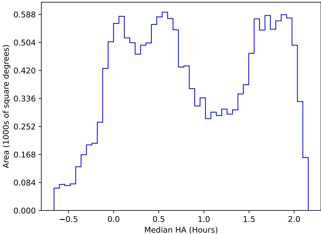
internal_u_expt60_nscale1.5v3.4_10yrs WFD r band: Median HA
