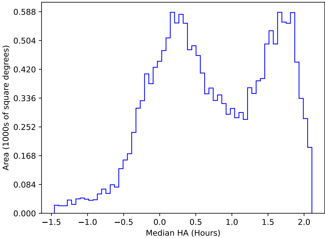
internal_u_expt60_nscale1.5v3.4_10yrs WFD g band: Median HA
