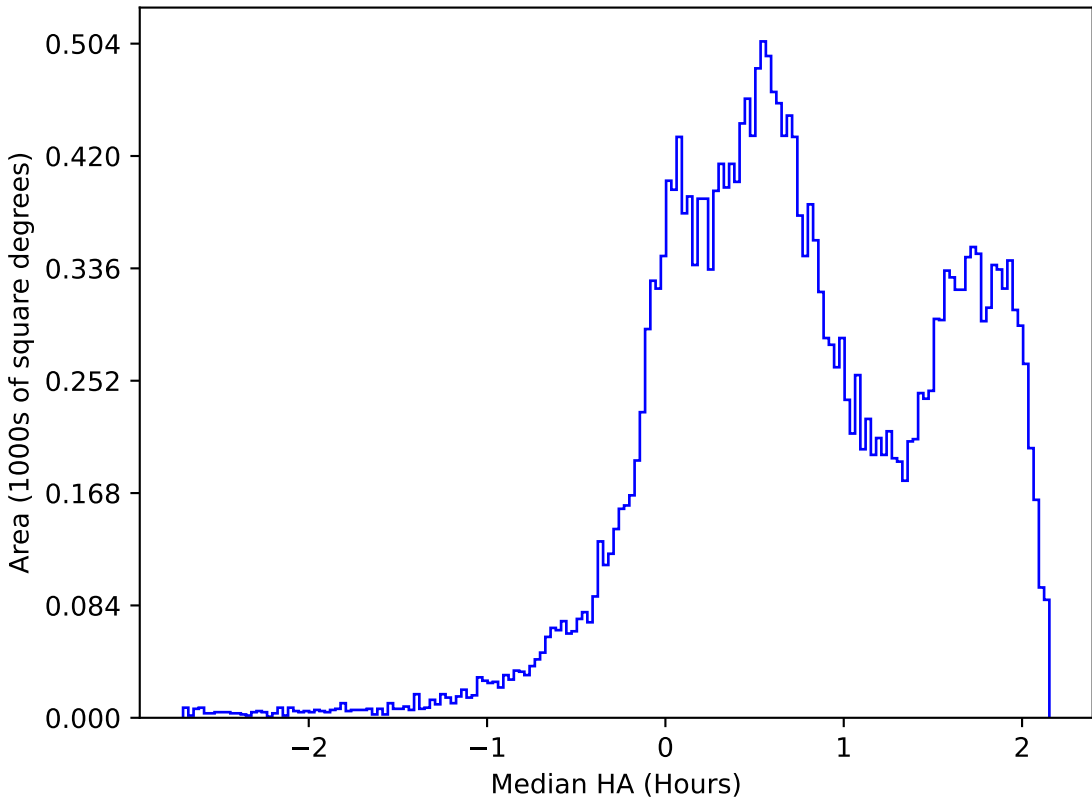
internal_u_expt60_nscale1.5v3.4_10yrs All sky r band: Median HA
