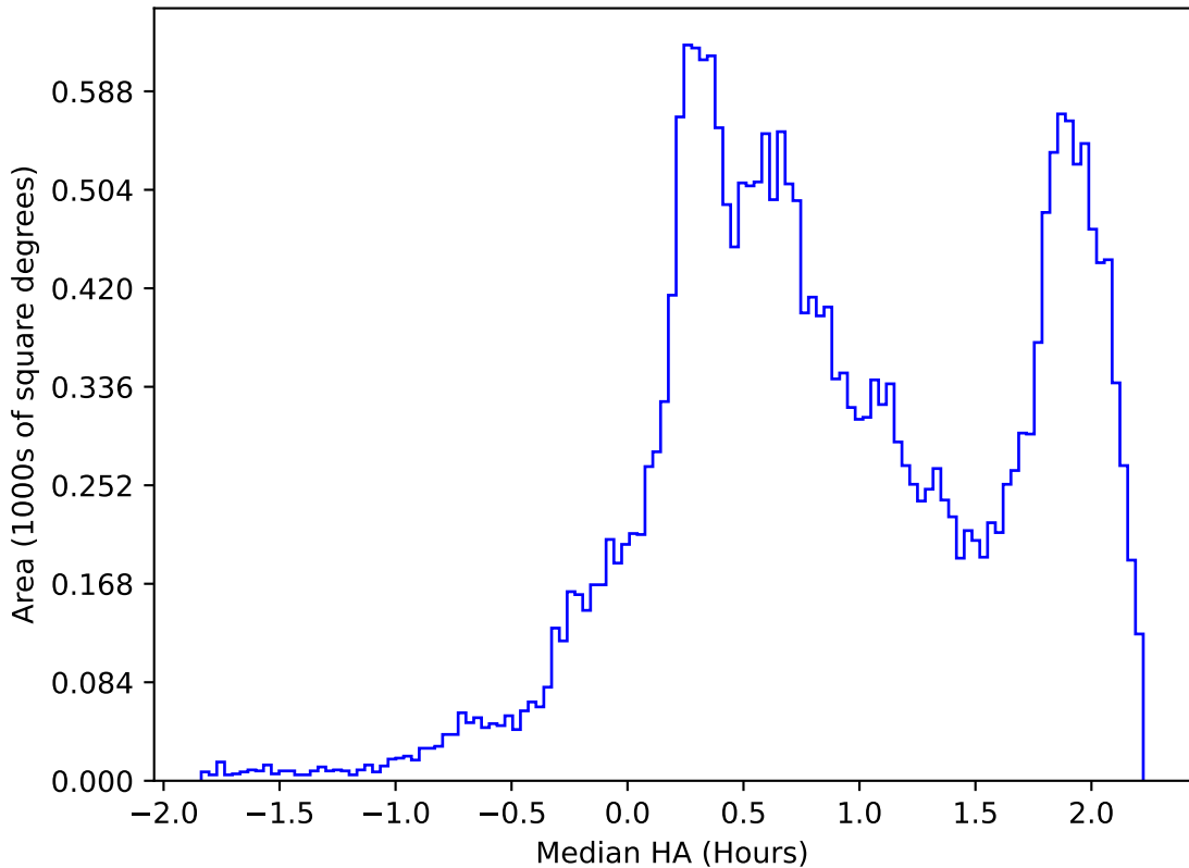
internal_u_expt60_nscale1.5v3.4_10yrs All sky all bands: Median HA
