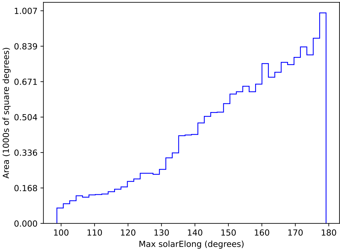
internal_u_expt60_nscale1.5v3.4_10yrs WFD y band: Max solarElong
