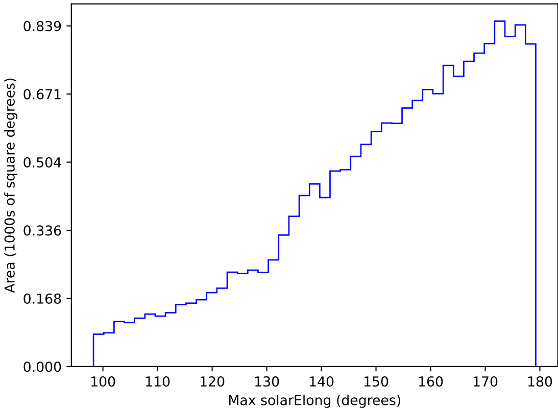
internal_u_expt60_nscale1.5v3.4_10yrs WFD u band: Max solarElong
