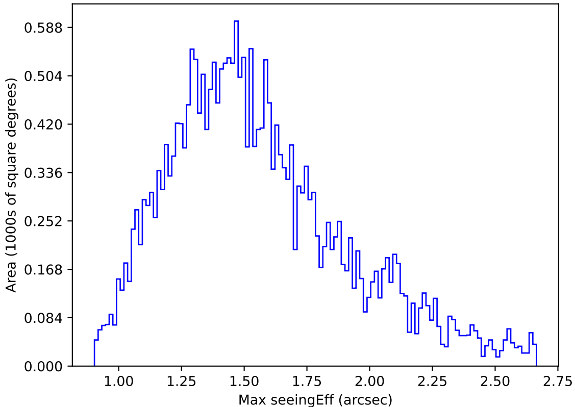
internal_u_expt60_nscale1.5v3.4_10yrs Yr 1 g band: Max seeingEff
