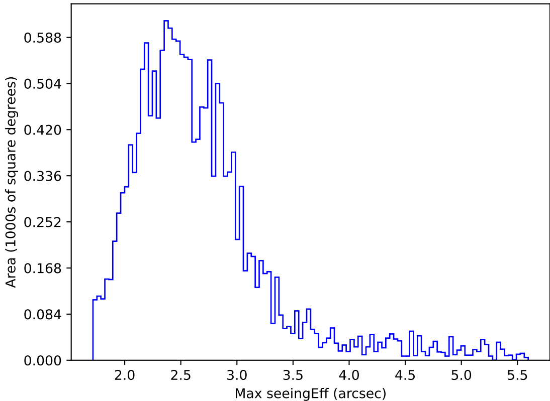
internal_u_expt60_nscale1.5v3.4_10yrs WFD i band: Max seeingEff
