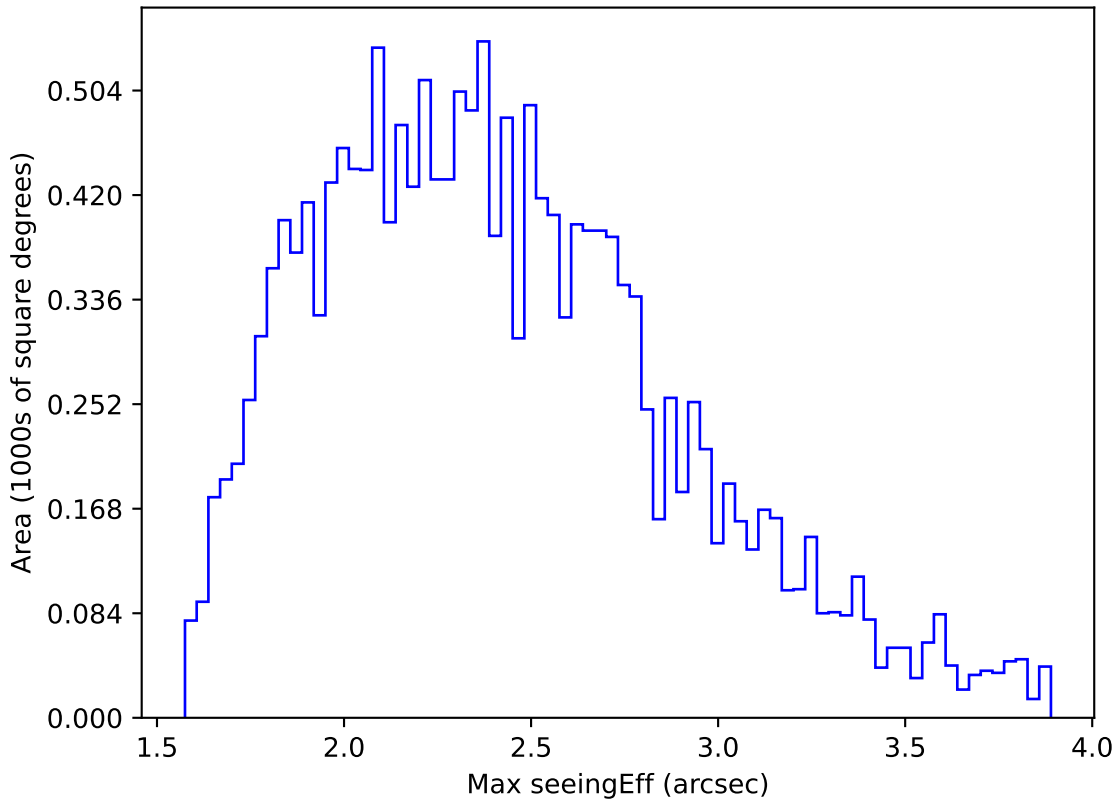
internal_u_expt60_nscale1.5v3.4_10yrs WFD g band: Max seeingEff
