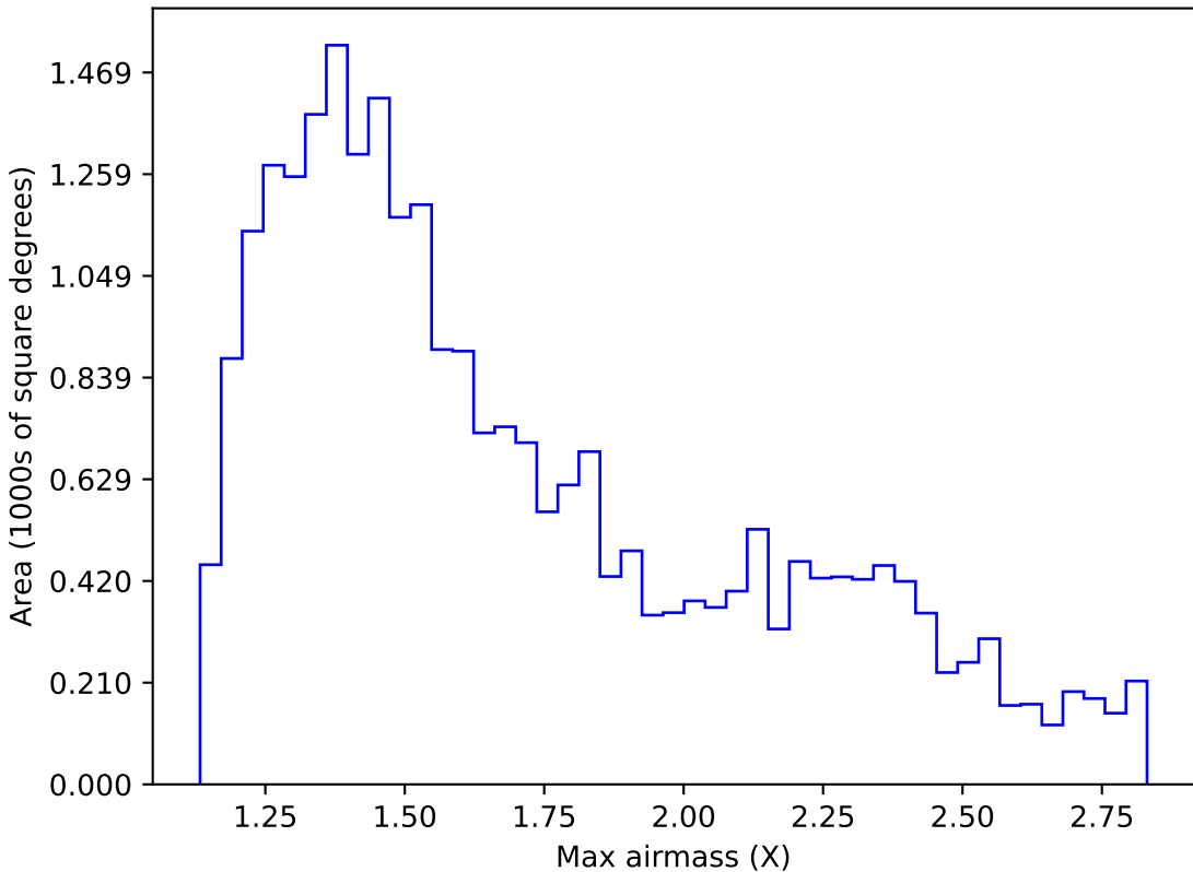
internal_u_expt60_nscale1.5v3.4_10yrs Yr 1 z band: Max airmass
