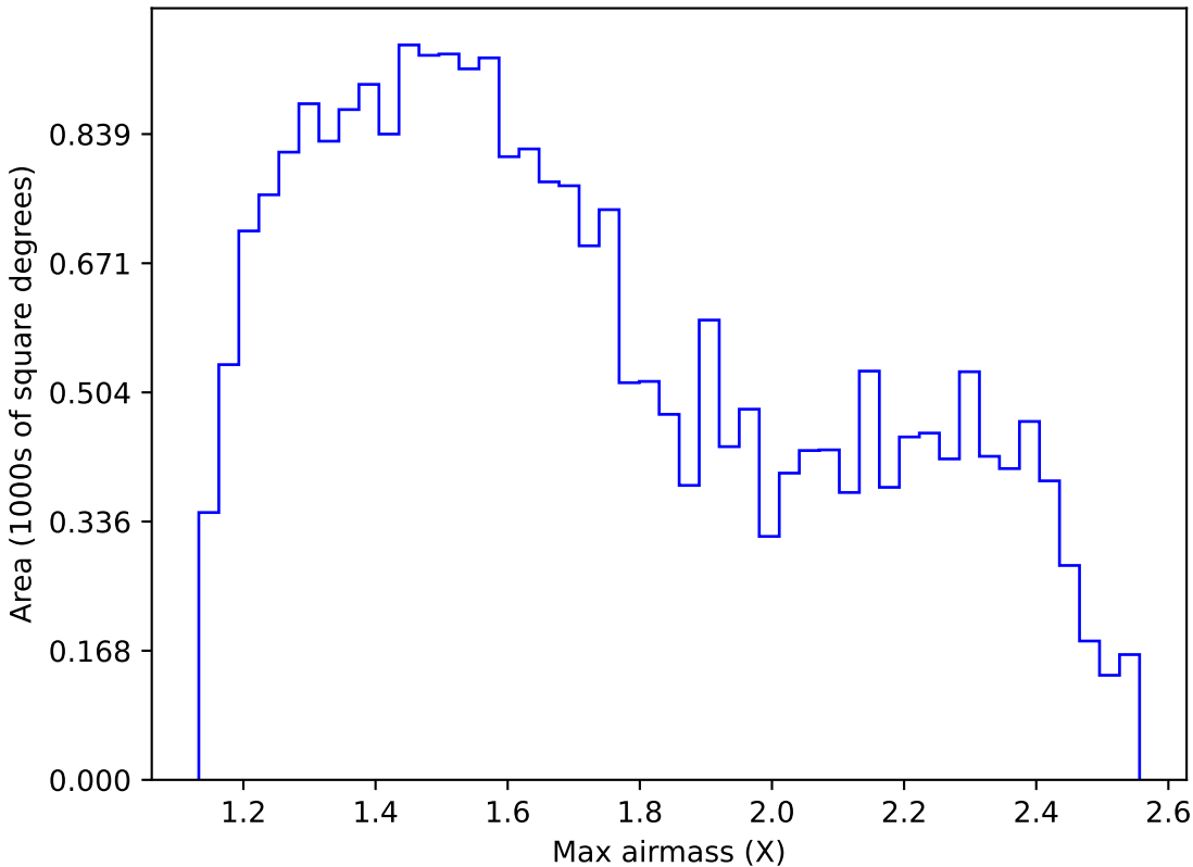
internal_u_expt60_nscale1.5v3.4_10yrs Yr 1 r band: Max airmass
