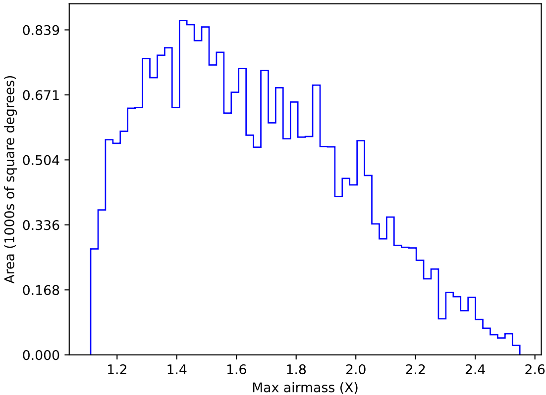
internal_u_expt60_nscale1.5v3.4_10yrs Yr 1 g band: Max airmass
