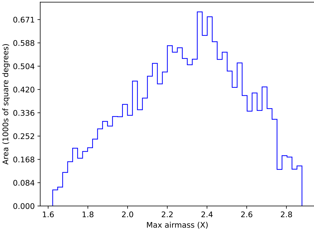
internal_u_expt60_nscale1.5v3.4_10yrs WFD y band: Max airmass
