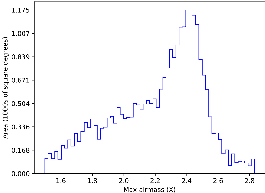
internal_u_expt60_nscale1.5v3.4_10yrs All sky r band: Max airmass
