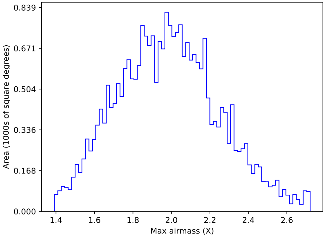
internal_u_expt60_nscale1.5v3.4_10yrs All sky g band: Max airmass
