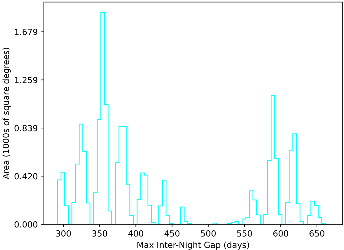
internal_u_expt60_nscale1.5v3.4_10yrs WFD u band: Max Inter-Night Gap
