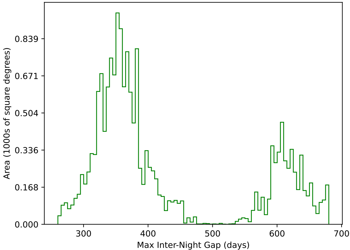
internal_u_expt60_nscale1.5v3.4_10yrs WFD g band: Max Inter-Night Gap
