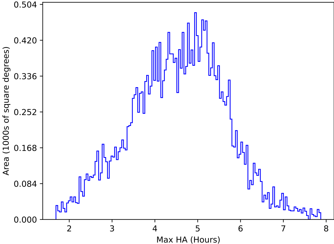
internal_u_expt60_nscale1.5v3.4_10yrs All sky z band: Max HA
