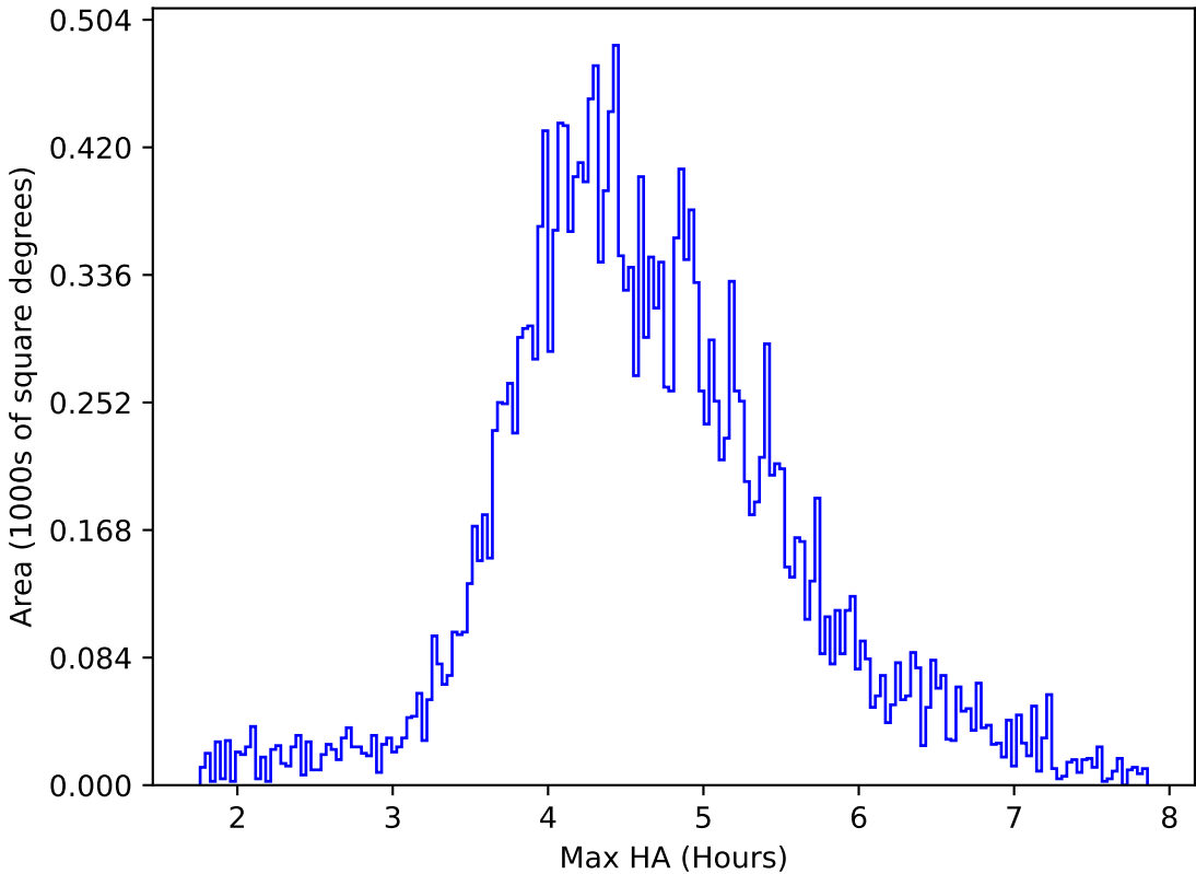
internal_u_expt60_nscale1.5v3.4_10yrs All sky y band: Max HA
