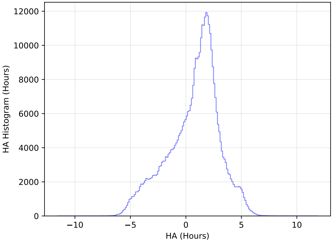
internal_u_expt60_nscale1.5v3.4_10yrs WFD z band: HA Histogram
