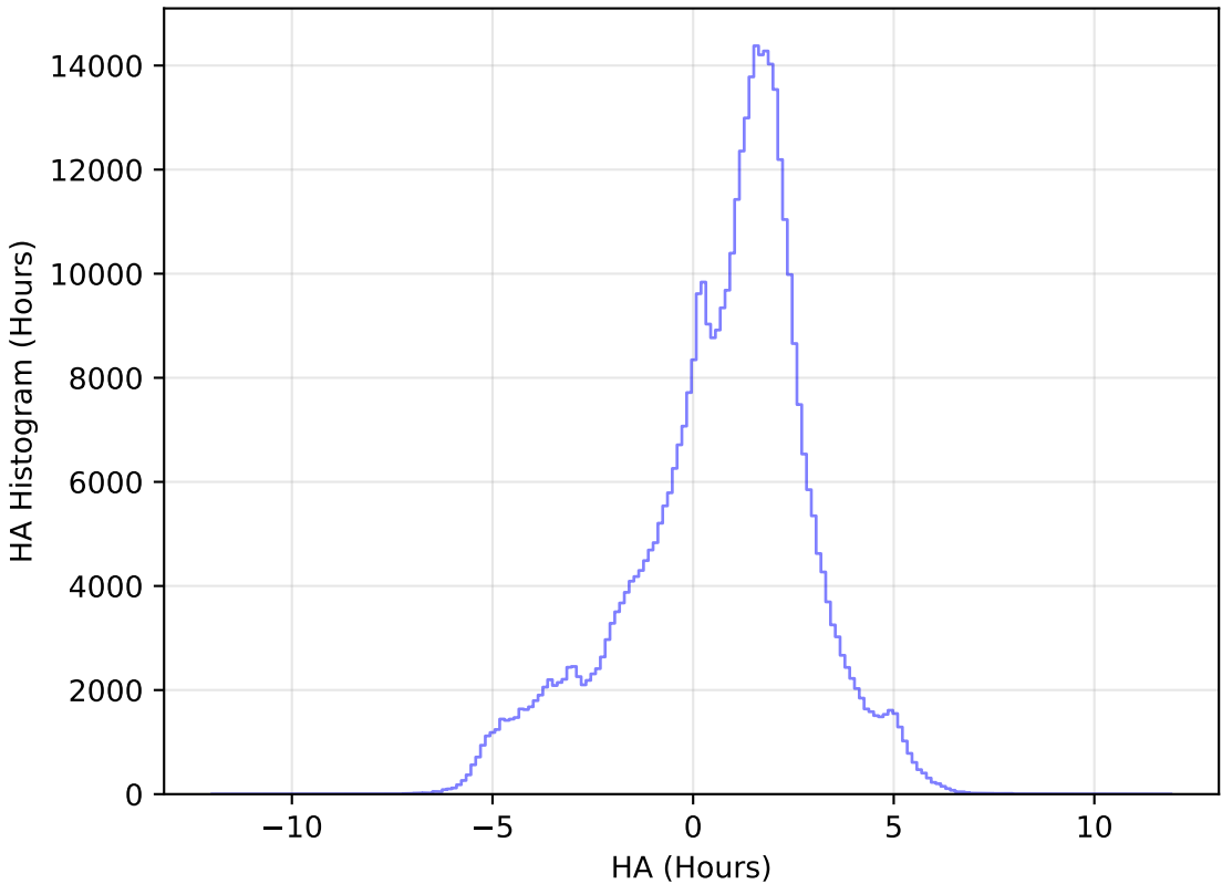
internal_u_expt60_nscale1.5v3.4_10yrs WFD i band: HA Histogram
