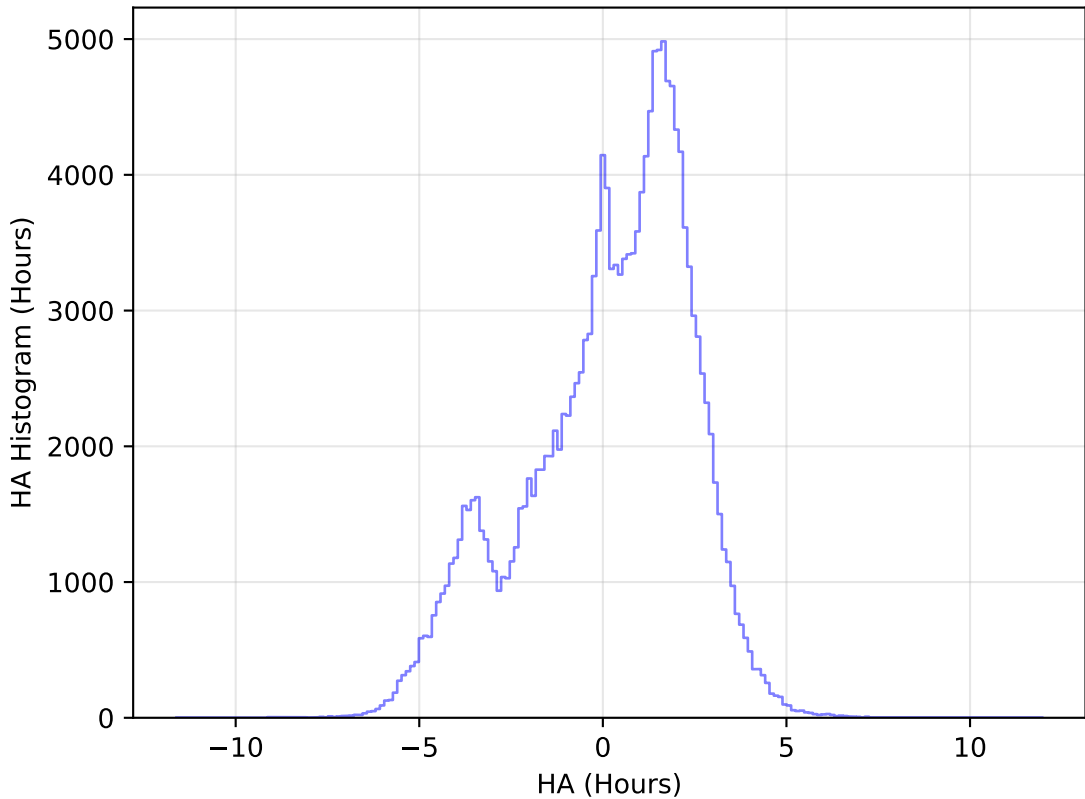
internal_u_expt60_nscale1.5v3.4_10yrs WFD g band: HA Histogram
