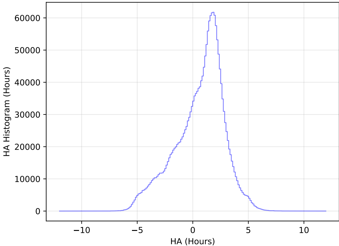
internal_u_expt60_nscale1.5v3.4_10yrs WFD all bands: HA Histogram
