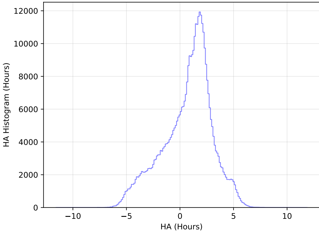
internal_u_expt60_nscale1.5v3.4_10yrs All sky z band: HA Histogram
