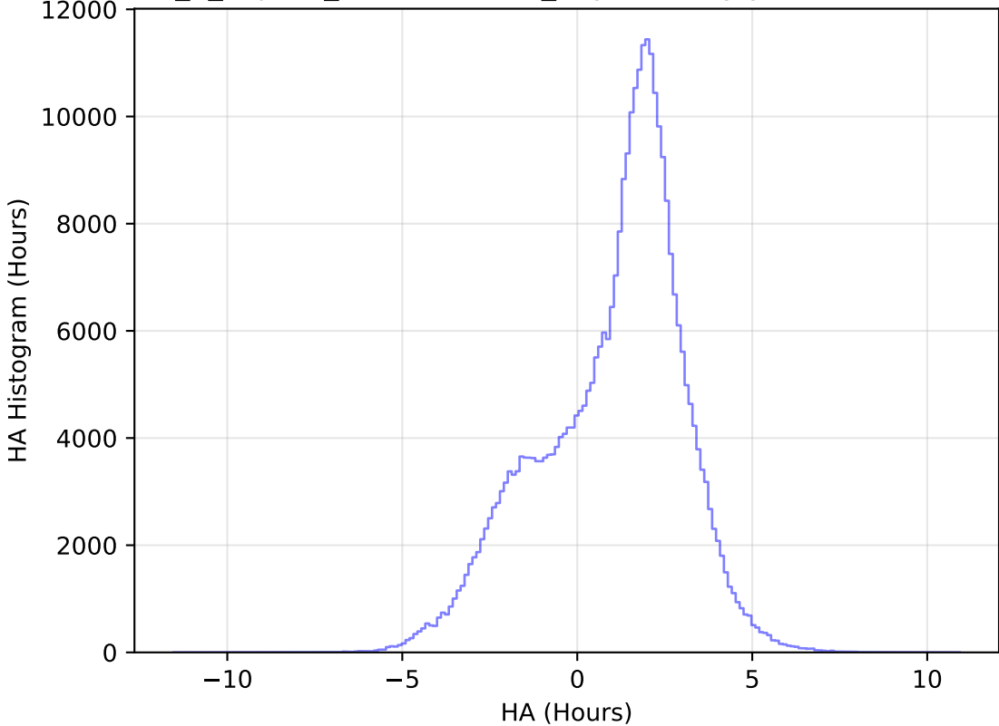
internal_u_expt60_nscale1.5v3.4_10yrs All sky y band: HA Histogram
