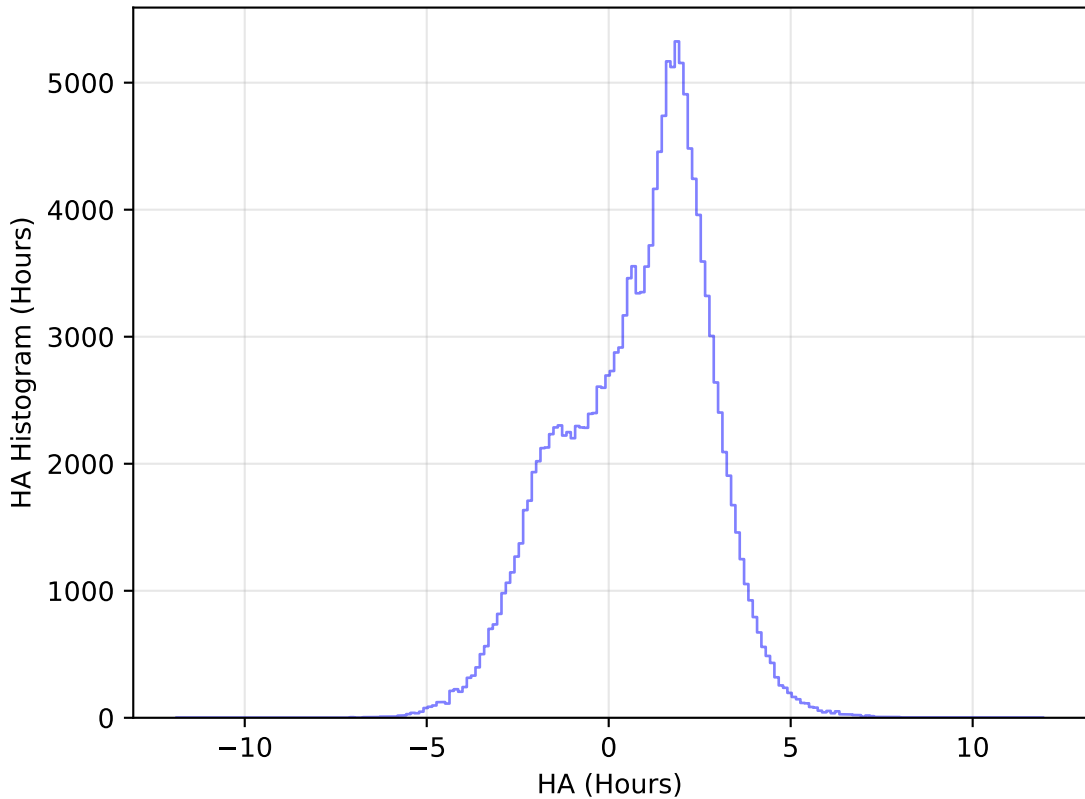
internal_u_expt60_nscale1.5v3.4_10yrs All sky u band: HA Histogram
