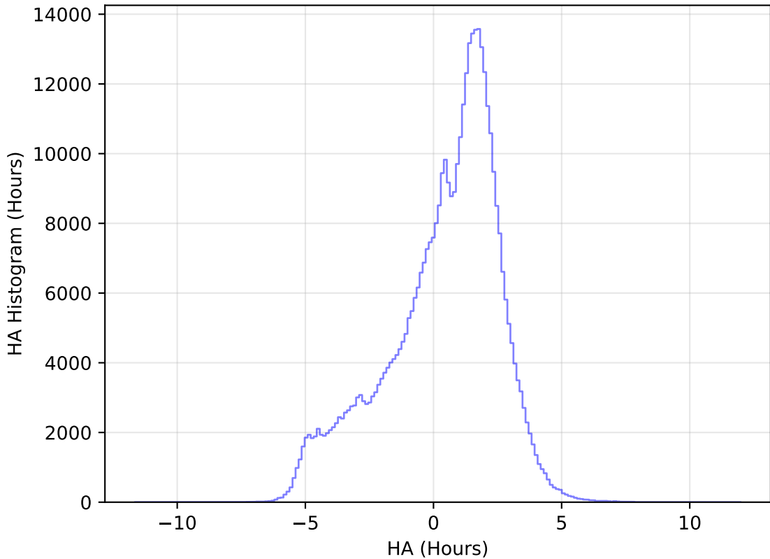
internal_u_expt60_nscale1.5v3.4_10yrs All sky r band: HA Histogram
