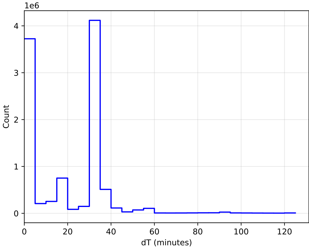
internal_u_expt60_nscale1.5v3.4_10yrs WFD: DeltaT Histogram
