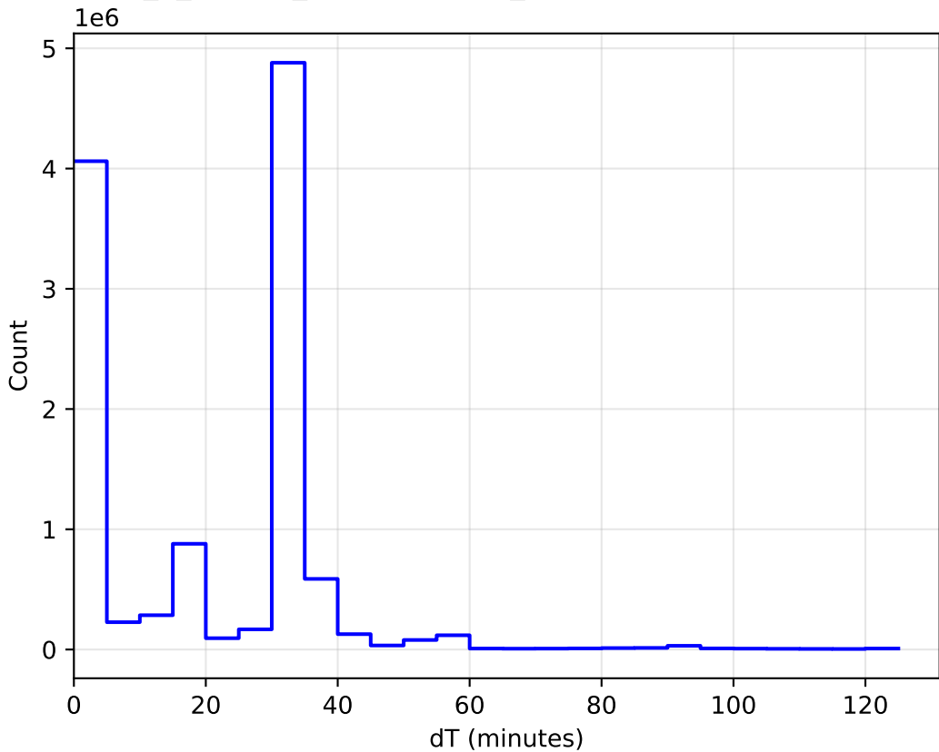
internal_u_expt60_nscale1.5v3.4_10yrs All sky: DeltaT Histogram
