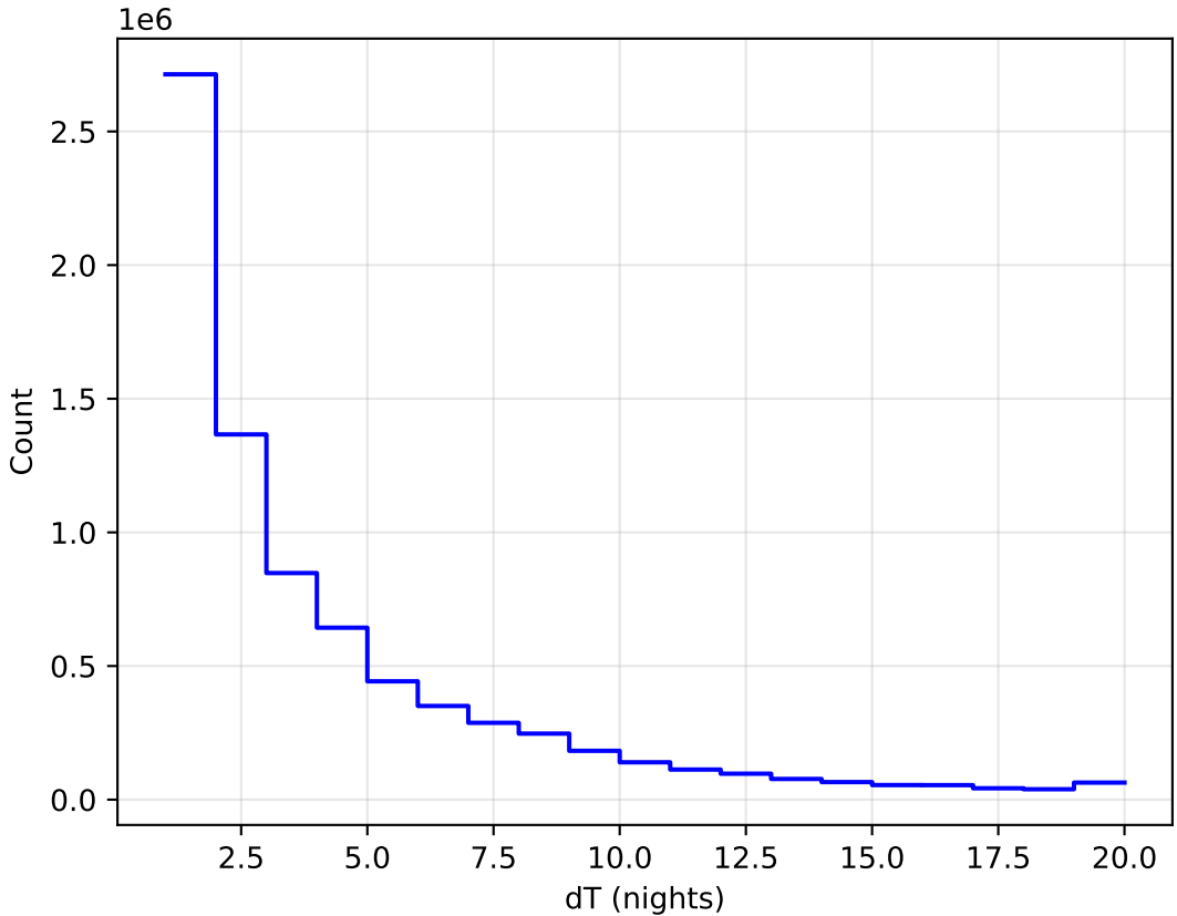
internal_u_expt60_nscale1.5v3.4_10yrs WFD all bands: DeltaNight Histogram
