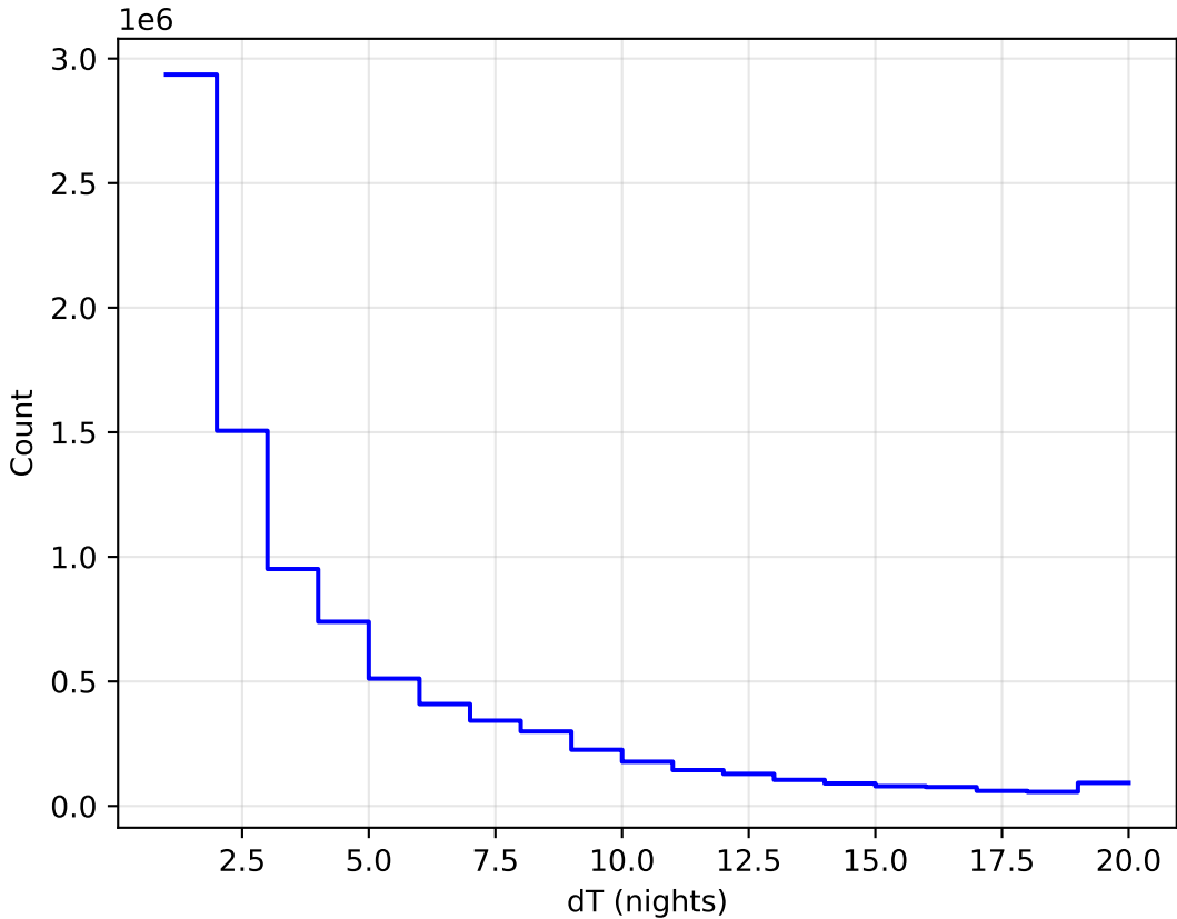
internal_u_expt60_nscale1.5v3.4_10yrs All sky all bands: DeltaNight Histogram
