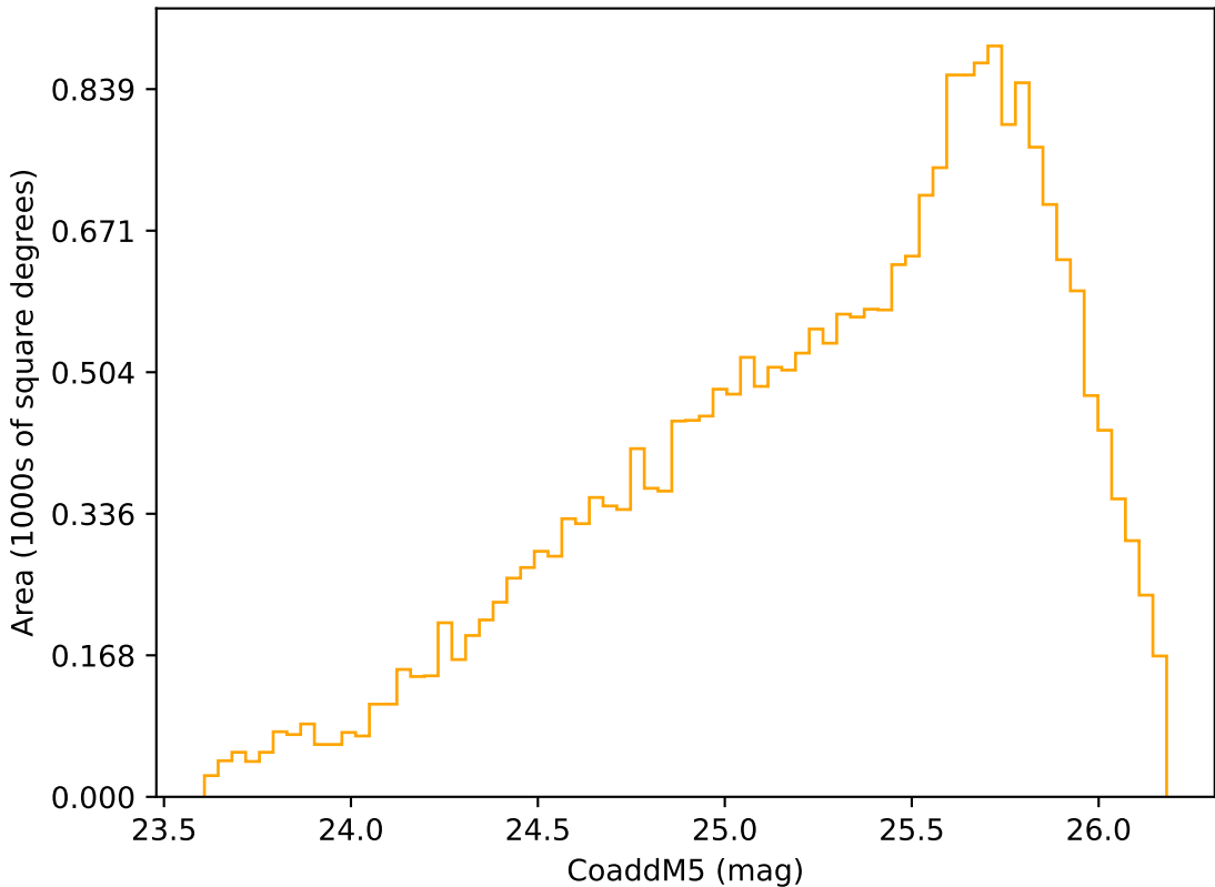
internal_u_expt60_nscale1.5v3.4_10yrs Yr 3-4 r band: CoaddM5
