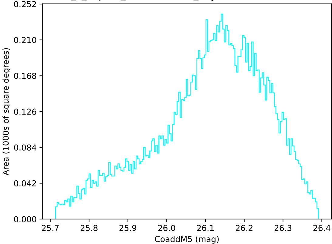
internal_u_expt60_nscale1.5v3.4_10yrs WFD u band: CoaddM5
