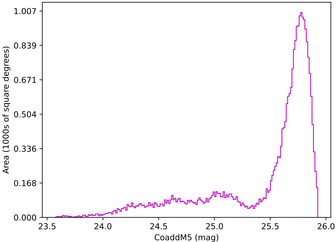
internal_u_expt60_nscale1.5v3.4_10yrs All sky z band: CoaddM5
