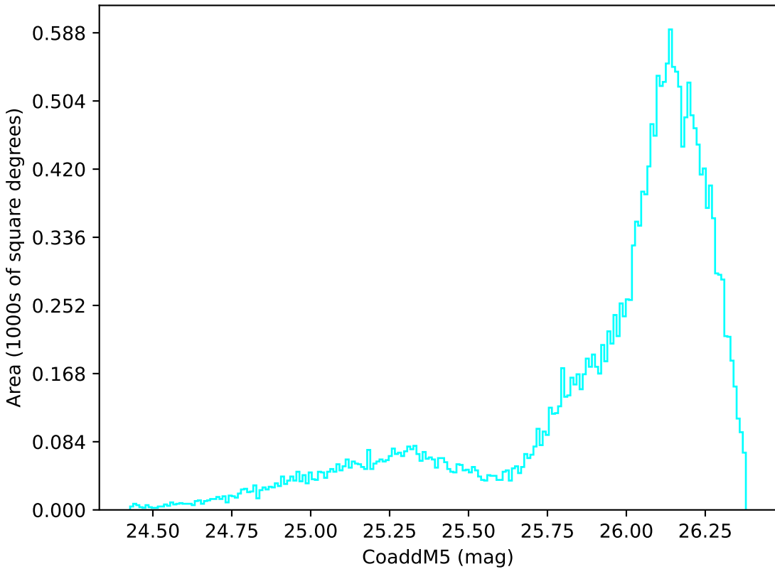
internal_u_expt60_nscale1.5v3.4_10yrs All sky u band: CoaddM5
